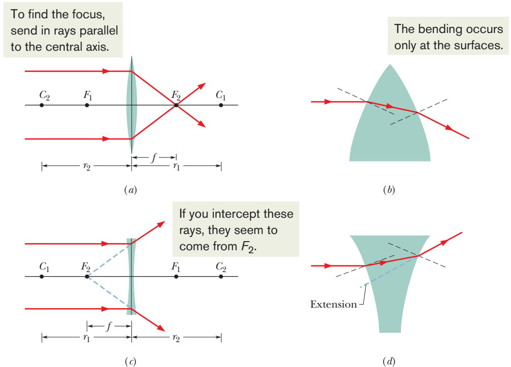
Figure 34-14 (a) Rays initially parallel to the central axis of a converging lens are made to converge to a real focal point F_2 by the lens. The lens is thinner than drawn, with a width like that of the vertical line through it. We shall consider all the bending of rays as occurring at this central line. (b) An enlargement of the top part of the lens of (a); normals to the surfaces are shown dashed. Note that both refractions bend the ray downward, toward the central axis. (c) The same initially parallel rays are made to diverge by a diverging lens. Extensions of the diverging rays pass through a virtual focal point F_2 . (d) An enlargement of the top part of the lens of (c). Note that both refractions bend the ray upward, away from the central axis.
