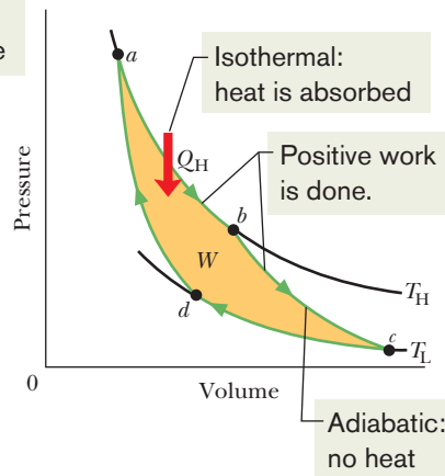
Stages of a Carnot engine
