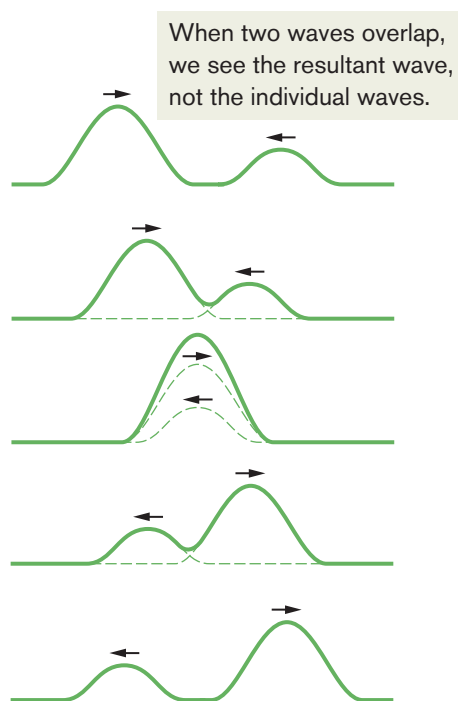
Figure 16-12 A series of snapshots that show two pulses traveling in opposite directions along a stretched string. The superposition principle applies as the pulses move through each other.
