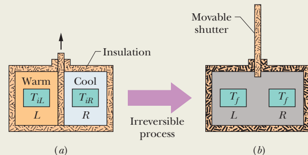
Figure 20-5 (a) In the initial state, two copper blocks L and R , identical except for their temperatures, are in an insulating box and are separated by an insulating shutter. (b) When the shutter is removed, the blocks exchange energy as heat and come to a final state, both with the same temperature T_f .
