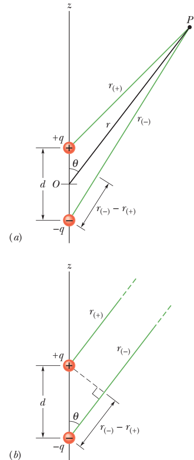
Figure 24-13 (a) Point P is a distance r from the midpoint O of a dipole. The line OP makes an angle \theta with the dipole axis. (b) If P is far from the dipole, the lines of lengths r_{(+)} and r_{(-)} are approximately parallel to the line of length r , and the dashed black line is approximately perpendicular to the line of length r_{(-)} .
