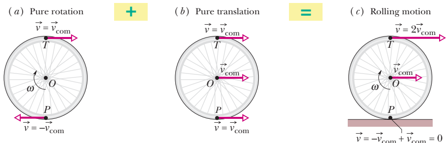
Figure 11-4 Rolling motion of a wheel as a combination of purely rotational motion and purely translational motion. (a) The purely rotational motion: All points on the wheel move with the same angular speed \omega . Points on the outside edge of the wheel all move with the same linear speed v = v_{\text{com}} . The linear velocities \vec{v} of two such points, at top ( T ) and bottom ( P ) of the wheel, are shown. (b) The purely translational motion: All points on the wheel move to the right with the same linear velocity \vec{v}_{\text{com}} . (c) The rolling motion of the wheel is the combination of (a) and (b).
