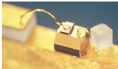
Figure 41-18 A junction laser developed at the AT&T Bell Laboratories. The cube at the right is a grain of salt.
