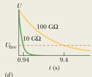
Figure 27-17 (a) A charged car and the pavement acts like a capacitor that can discharge through the tires. (b) The effective circuit of the car–pavement capacitor, with four tire resistances R_{\text{tire}} connected in parallel. (c) The equivalent resistance R of the tires. (d) The electric potential energy U in the car–pavement capacitor decreases during discharge.
