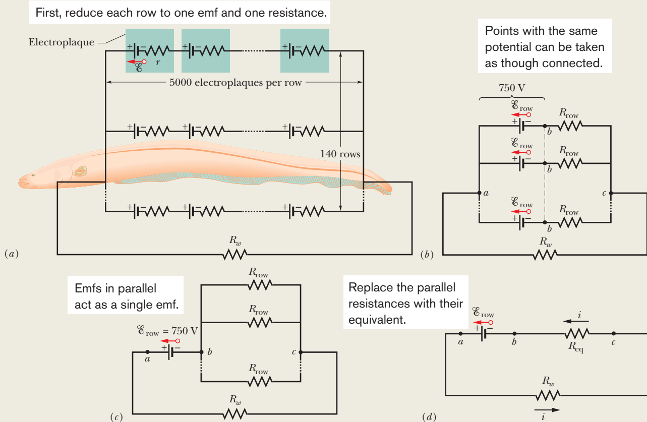
Figure 27-12 (a) A model of the electric circuit of an eel in water. Along each of 140 rows extending from the head to the tail of the eel, there are 5000 electroplaques. The surrounding water has resistance R_w . (b) The emf \mathcal{E}_{\text{row}} and resistance R_{\text{row}} of each row. (c) The emf between points a and b is \mathcal{E}_{\text{row}} . Between points b and c are 140 parallel resistances R_{\text{row}} . (d) The simplified circuit.
