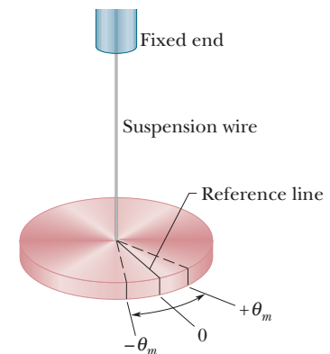
Figure 15-9 A torsion pendulum is an angular version of a linear simple harmonic oscillator. The disk oscillates in a horizontal plane; the reference line oscillates with angular amplitude \theta_m . The twist in the suspension wire stores potential energy as a spring does and provides the restoring torque.
