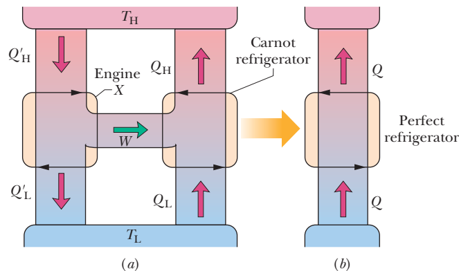
Figure 20-16 (a) Engine X drives a Carnot refrigerator. (b) If, as claimed, engine X is more efficient than a Carnot engine, then the combination shown in (a) is equivalent to the perfect refrigerator shown here. This violates the second law of thermodynamics, so we conclude that engine X cannot be more efficient than a Carnot engine.
